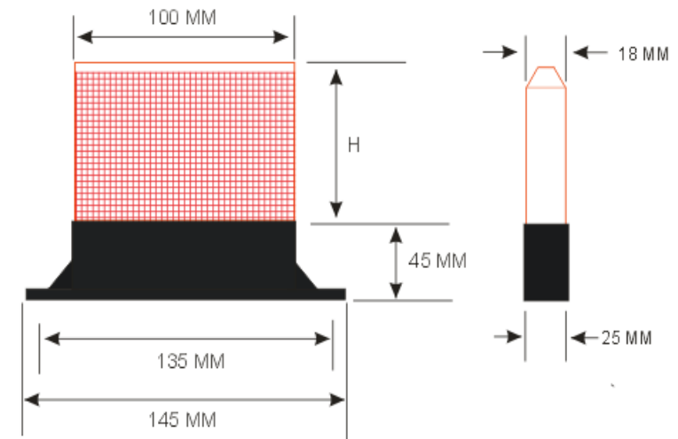
Product Dimension
